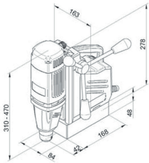
MABasic 400
