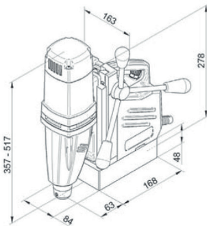
MABasic 450
