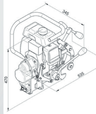
RailMAB 960
