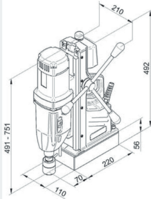
MAB 155
