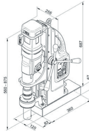
MAB 1300
