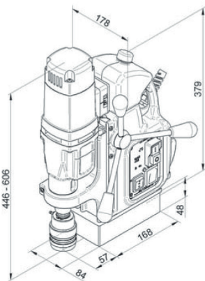
MAB 525
