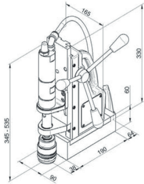
RailMAB 925
