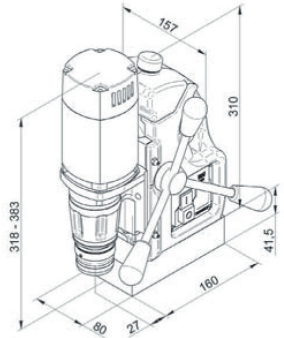
MAB 455
