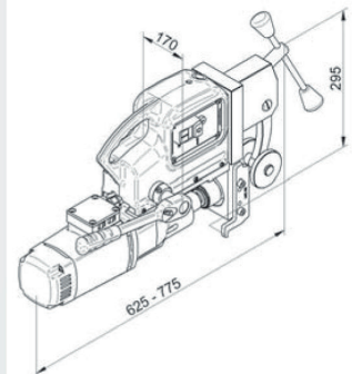
RailMAB 960
