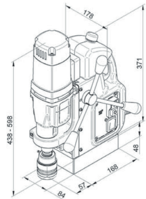
MAB 455
