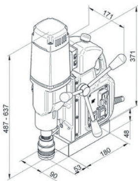
MAB 525
