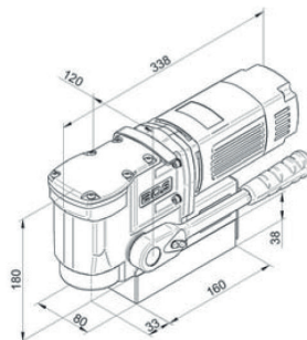
AutoMAB 350
